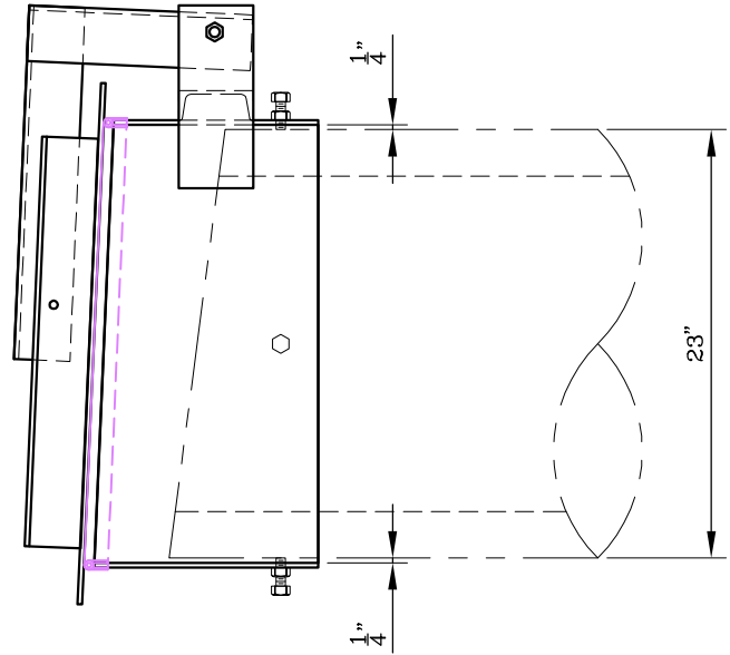
SIDE ELEVATION
